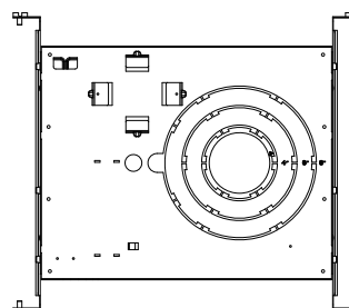
DLPLATE/C3468R/NB Mounting plate with nailer bar
