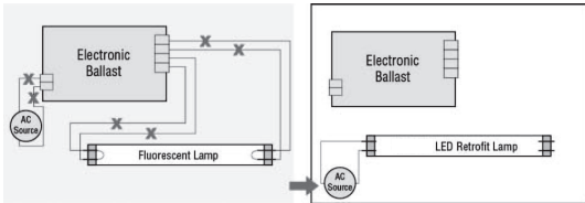
Fig. 3 - Retrofit with One Lamp
