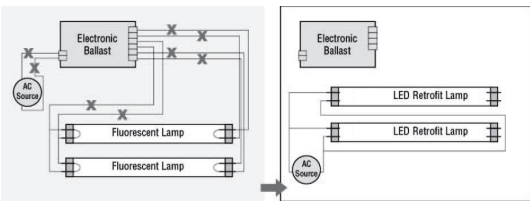
Fig. 4 - Retrofit with Two Lamps
