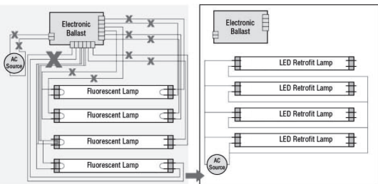
Fig. 5 - Retrofit with Three/Four Lamps
