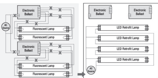
Fig. 6 - Retrofit with Three/Four Lamps & Two Ballasts
