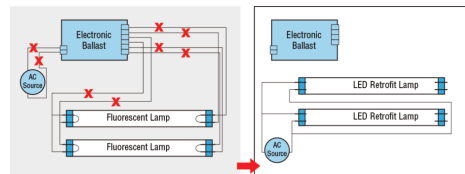
Fig:4 - Retrofit with Two Lamps
