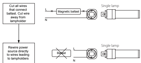
Diagram 2 – Magnetic ballast fixture wiring modification
