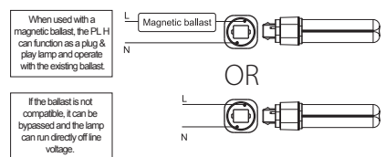
Diagram 3 – Magnetic ballast fixture wiring modification
