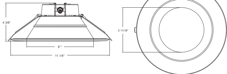
CRLEDFA-10R-43S-9CCT-UNV-WS
