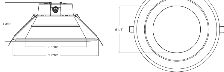
CRLEDFA-8R-33S-9CCT-UNV-WS CRLEDFA-8R-22S-9CCT-UNV-WS
