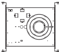
DLPLATE/C3468R/NB Mounting plate with nailer bar
