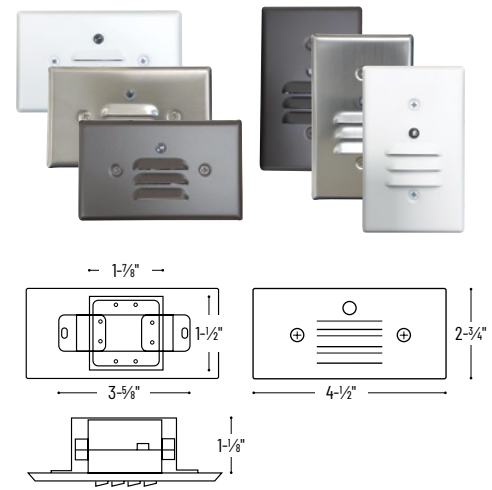
NSW-6619PC Louver with Lens (includes horizontal and vertical louver)
