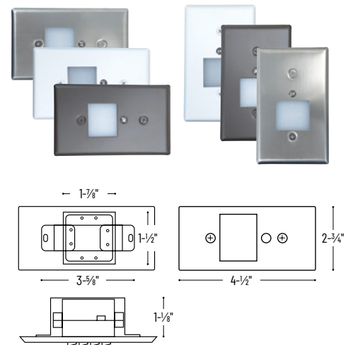
NSW-6629PC Lensed (can be mounted horizontally or vertically)
