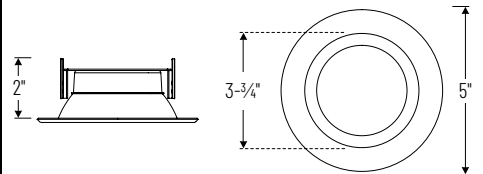
NOXAC-431 / NOX-4OR-W White Oversize Ring
