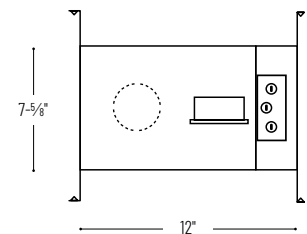
Ceiling Cut-Out
