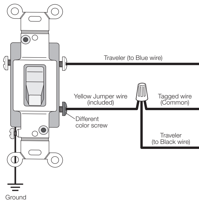
3-Way Mechanical Switch Wiring with Dimmer Sensor
