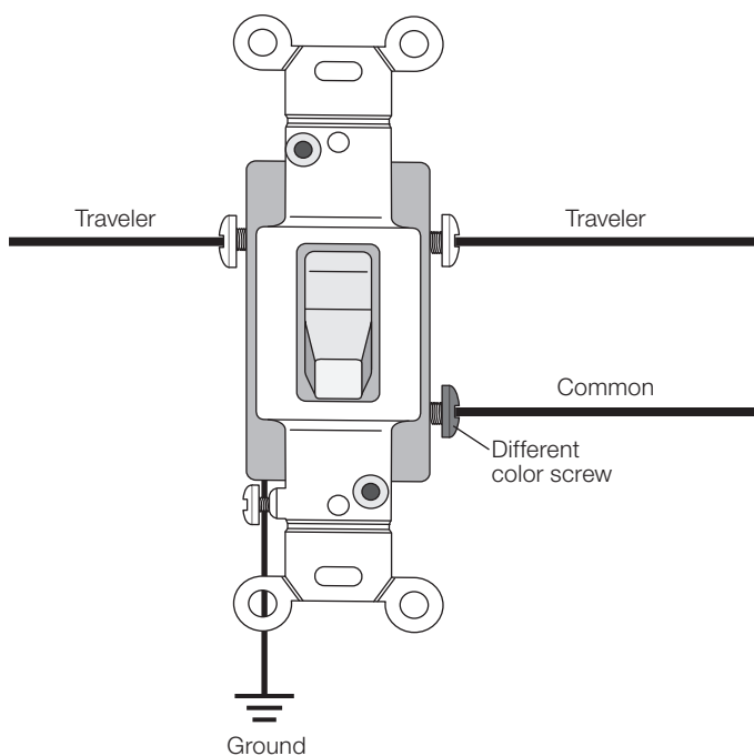
Traditional 3-Way Mechanical Switch Wiring
