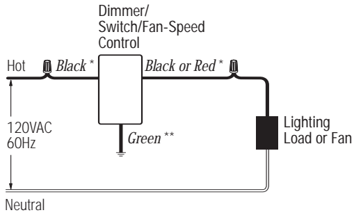
Wiring Diagram 10 Single-Pole Wiring
