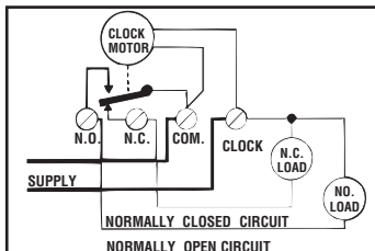
WIRING DIAGRAM
